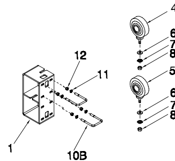
881 HAY HIKER with SIDE RAILS
